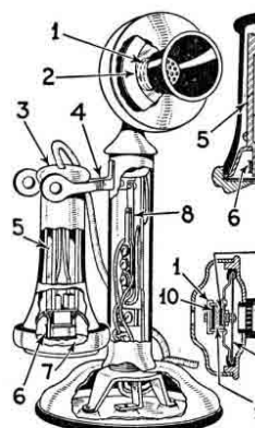
View, partly sectional, of a typical Telephone, with cross-sectional vi
