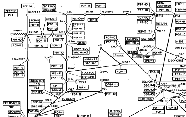
ARPANET LOGICAL MAP, MARCH 1977
